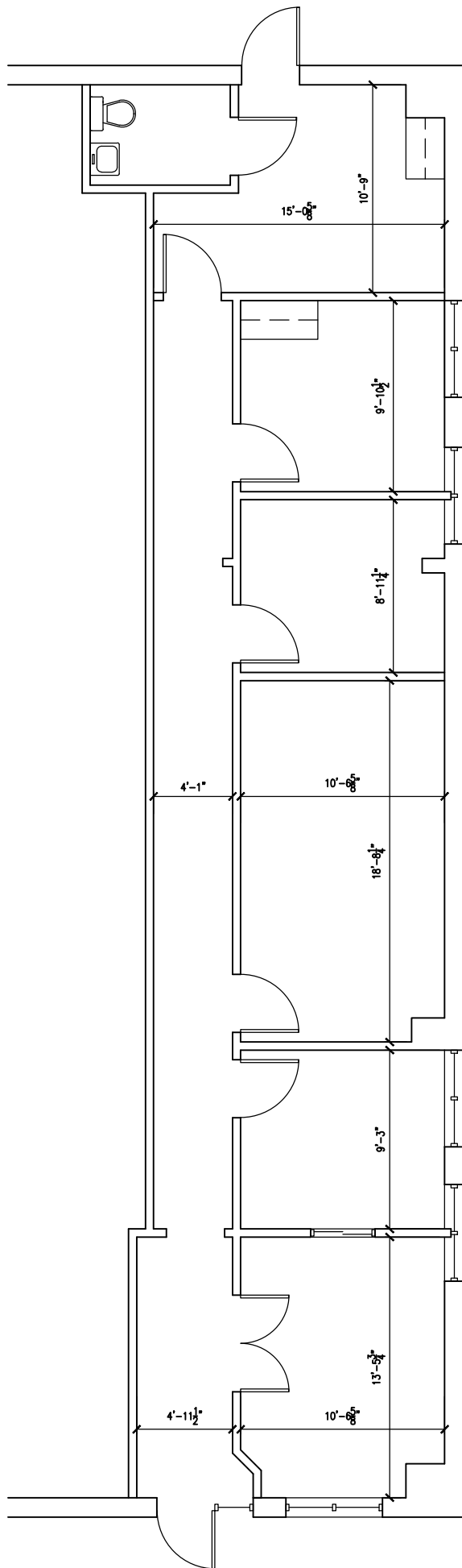
01 FLOOR PLAN FOR 4907 SANDHILL, SUITE F 1/8" = 1'-0" 12/5/2018
